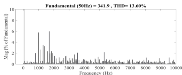
APODSPWM
