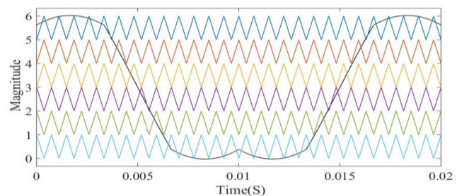
PODSVPWM
