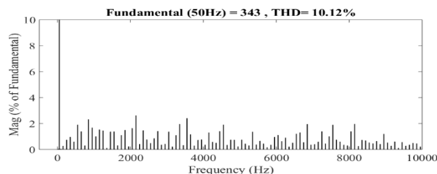
PDSPWM-Trapezoidal
