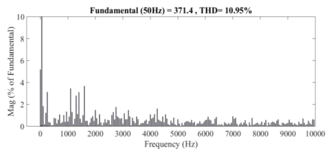
PODSVPWM
