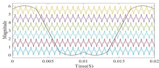
PDSVPWM- Trapezoidal
