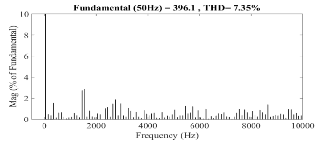
PDSVPWM-Trapezoidal
