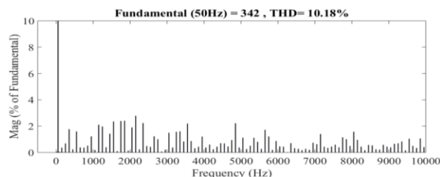
PDSPWM
