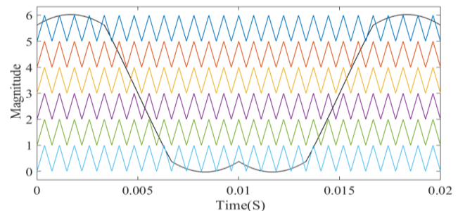
PDSVPWM
