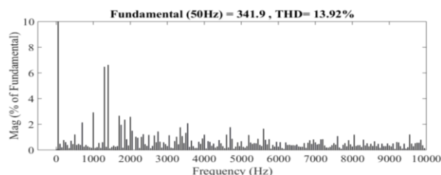
PODSPWM
