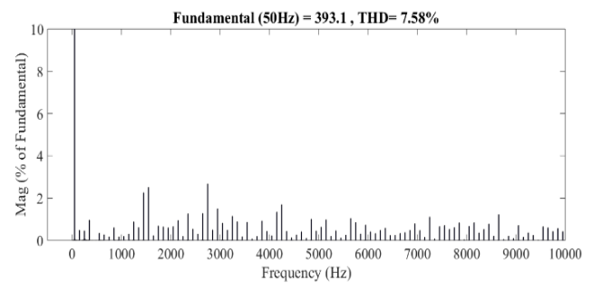
PDSVPWM
