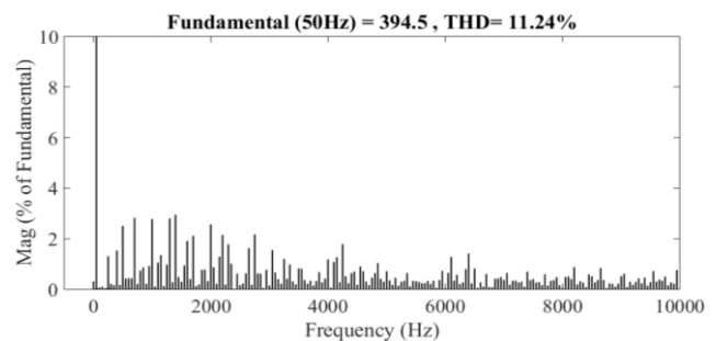
APODSVPWM
