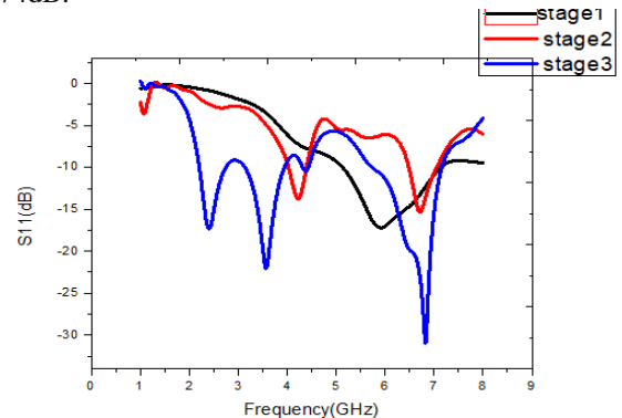
Fig. 3.a. S11 characteristics for different antenna configurations.
