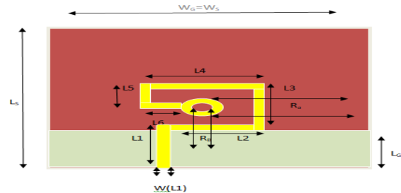
Fig.1.a . Feeding structure (stage4)
