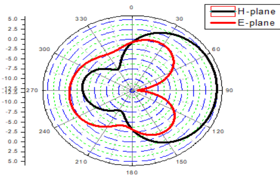
Fig. 6. Radiation pattern at 3.5GHz
