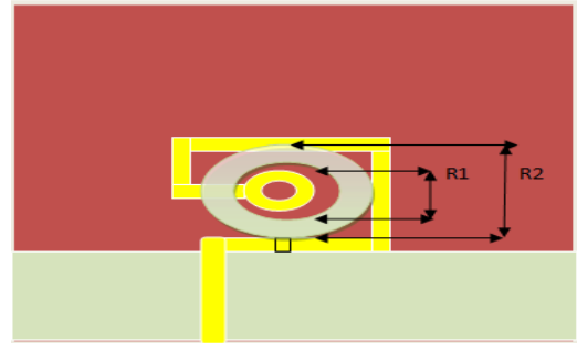
Fig.2.c. Proposed Antenna (stage3)
