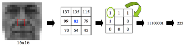
Figure 3: LBP Conversion to Binary
