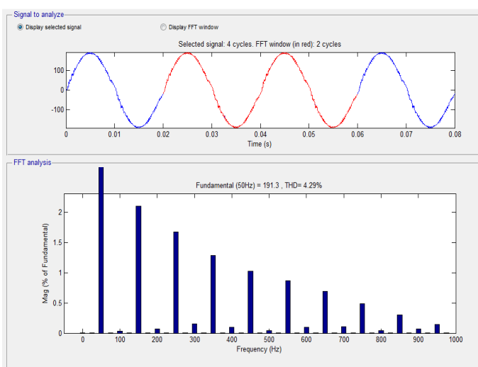
Fig.16 THD of proposed topology with filter
