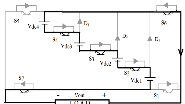
(a) V_{out} = V_{dc4} + V_{dc3} + V_{dc2} + V_{dc1}
