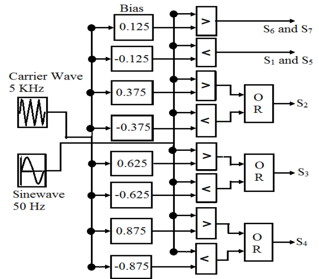
(a) SPWM pulse logic block
