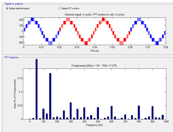
Fig.15 THD of proposed topology without filter
