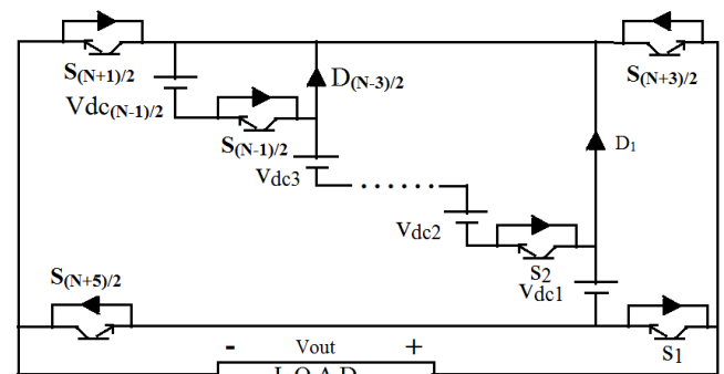
Fig.1 (a)-(d) Existing multilevel Inverter
