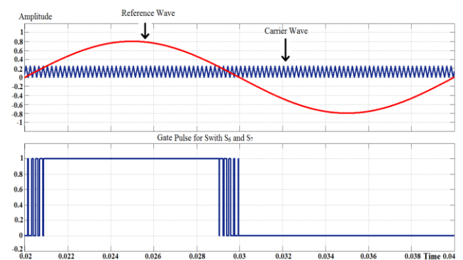
Fig.11 Pulse generation for switch S_6 and S_7
