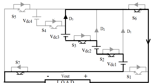
(b) V_{out} = V_{dc3} + V_{dc2} + V_{dc1}
