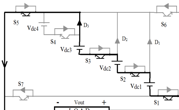
(c) V_{out} = -V_{dc3} - V_{dc2} - V_{dc1}
