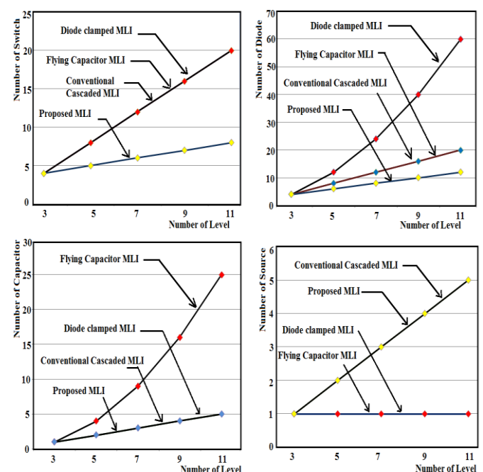
Fig.17 Graphs between numbers of power devices versus number of Levels
