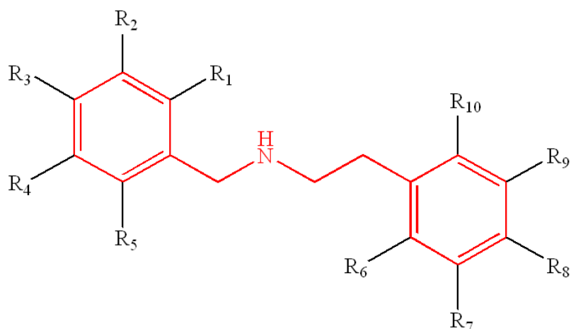
Figure 6. Schematic representation of the molecular structure of NBOMe-like substances.
