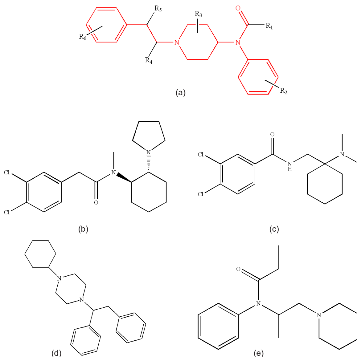
Figure 7. Schematic representation of the molecular structure of (a) Fentanyl-like substances, (b) U-50488, (c) AH-7921, (d) MT-45, and (e) Fenampromide.
