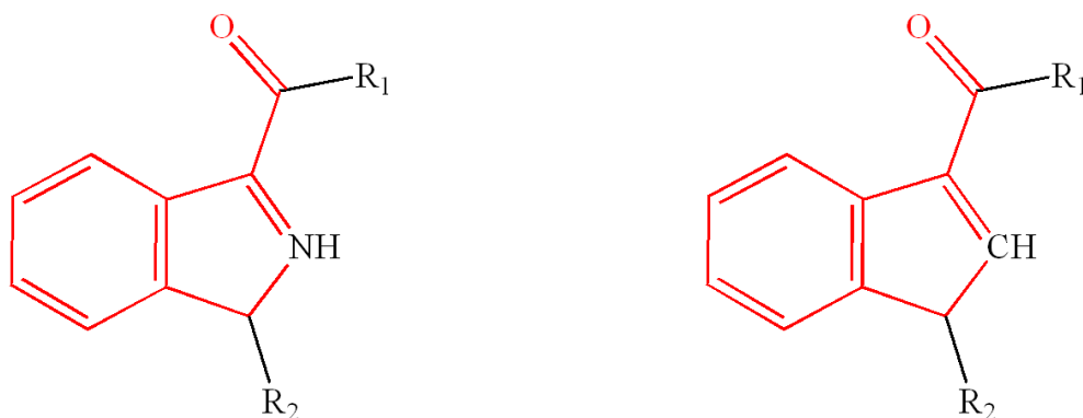
Figure 5. Schematic representation of the molecular structure of synthetic cannabinoid-like substances.
