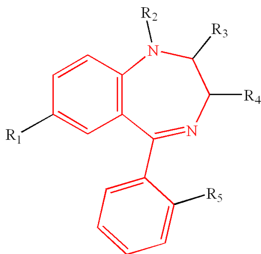
Figure 8. The classical structure of benzodiazepines is based on a 5-aryl-1,4-benzodiazepine structure. “R” labels denote common locations of side chains, which give different benzodiazepines their unique properties [44].
