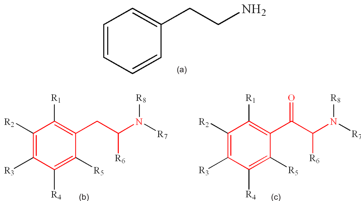
Figure 4. Schematic representation of the molecular structures of (a) Phenylethylamine, (b) Amphetamine-like substances, and (c) Cathinone-like substances.
